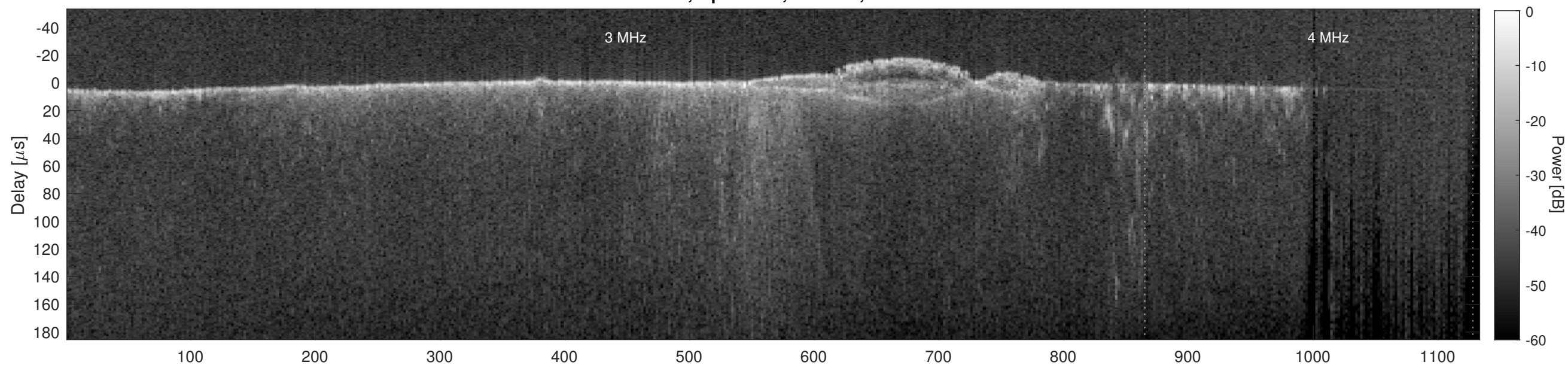
Orbit 11935, Cluttergram
