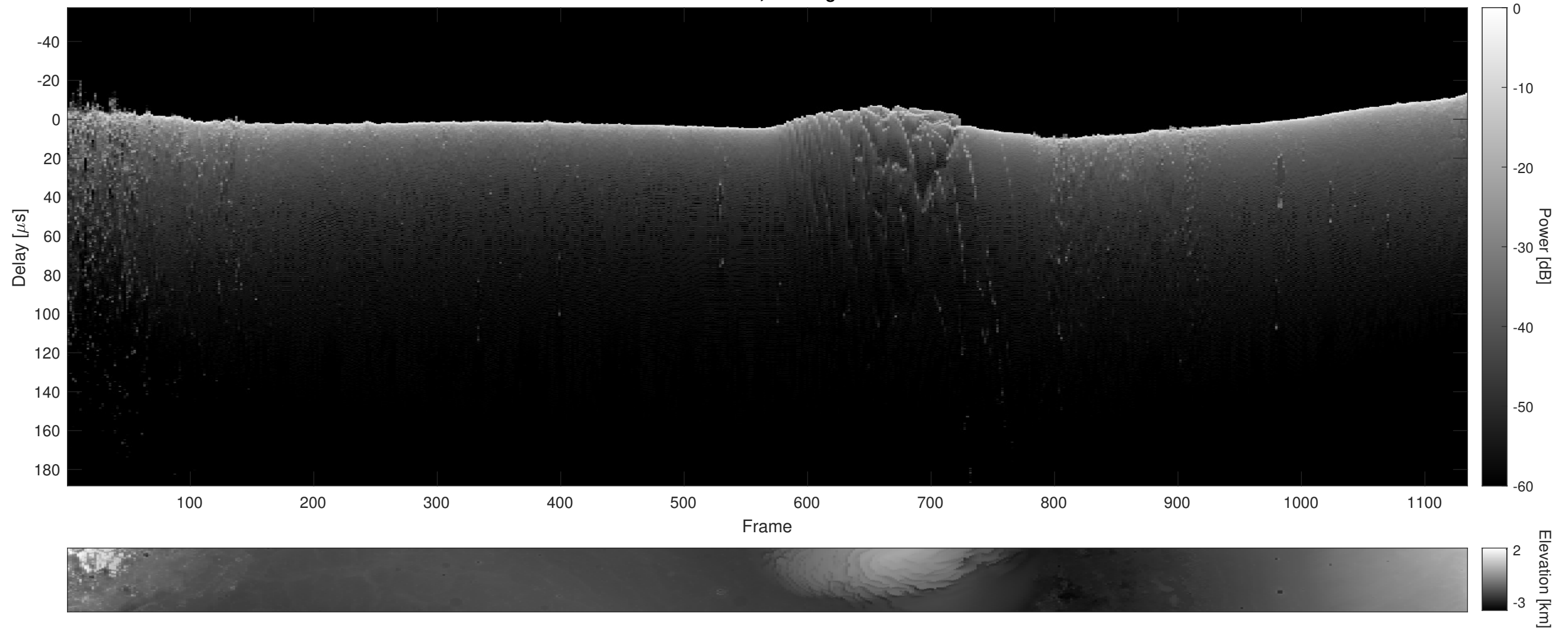
Orbit 11936, Cluttergram
