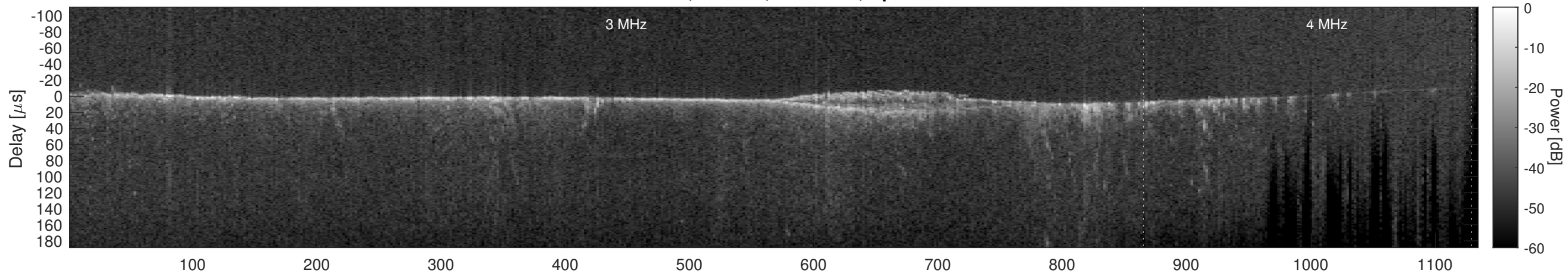
Orbit 11936, Cluttergram
