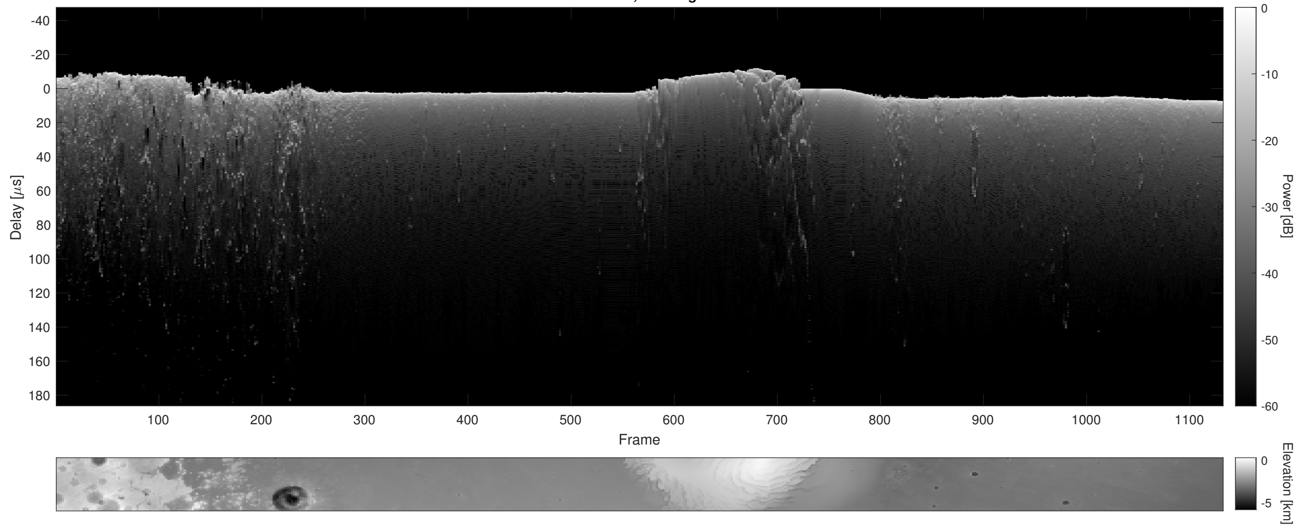
Orbit 11940, Cluttergram
