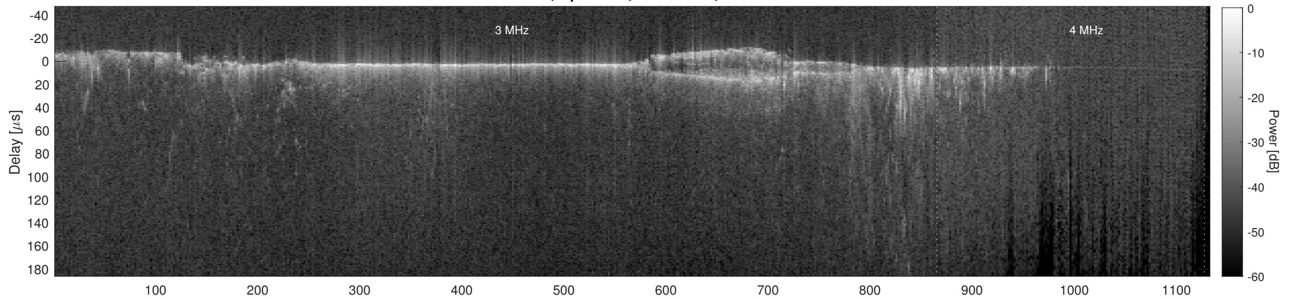
Orbit 11940, Cluttergram
