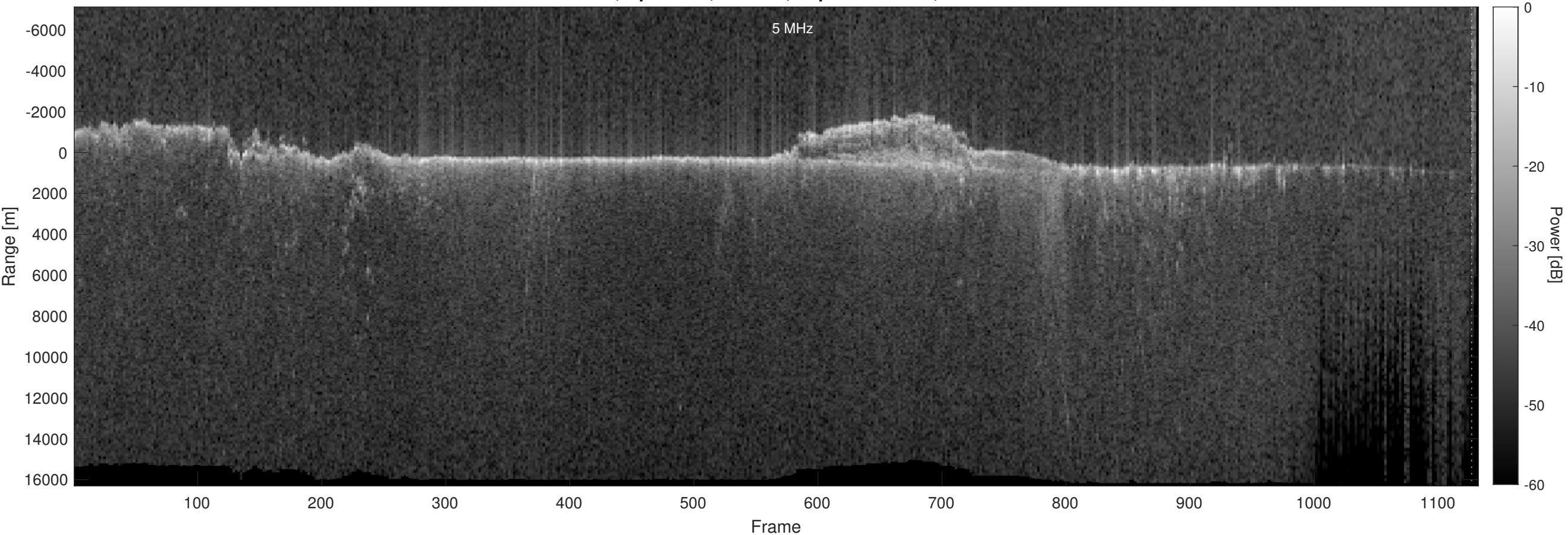
Orbit 11940, Optimized, Window, Depth-Corrected, Channel 2
