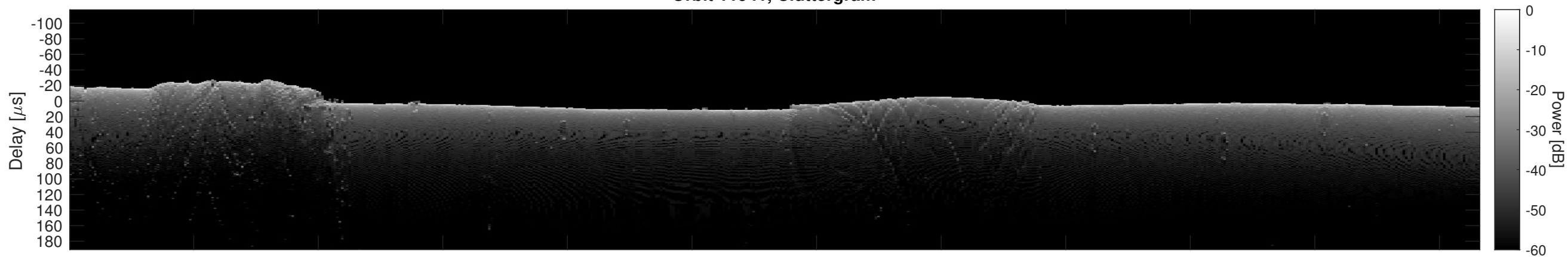
Orbit 11941, Cluttergram
