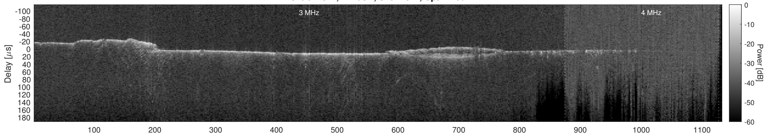
Orbit 11941, Cluttergram
