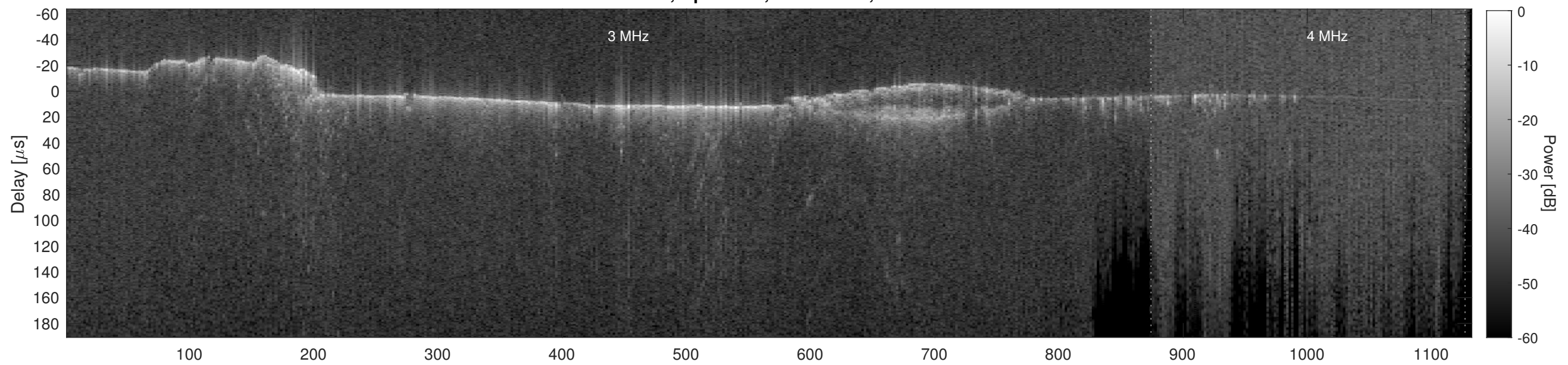
Orbit 11941, Cluttergram
