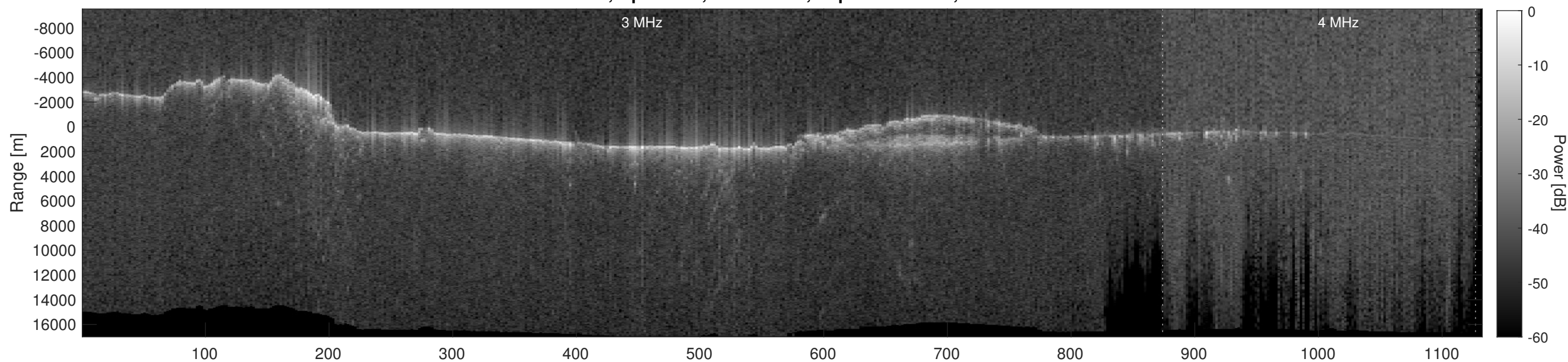
Orbit 11941, Depth-Corrected Cluttergram
