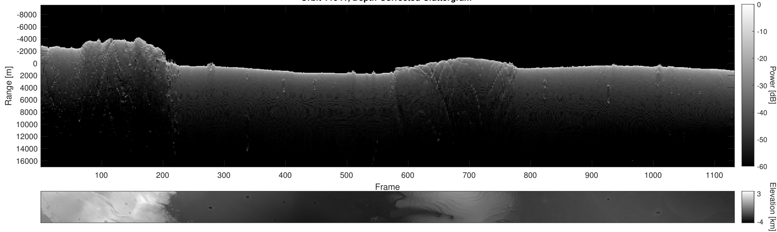
Orbit 11941, Depth-Corrected Cluttergram
