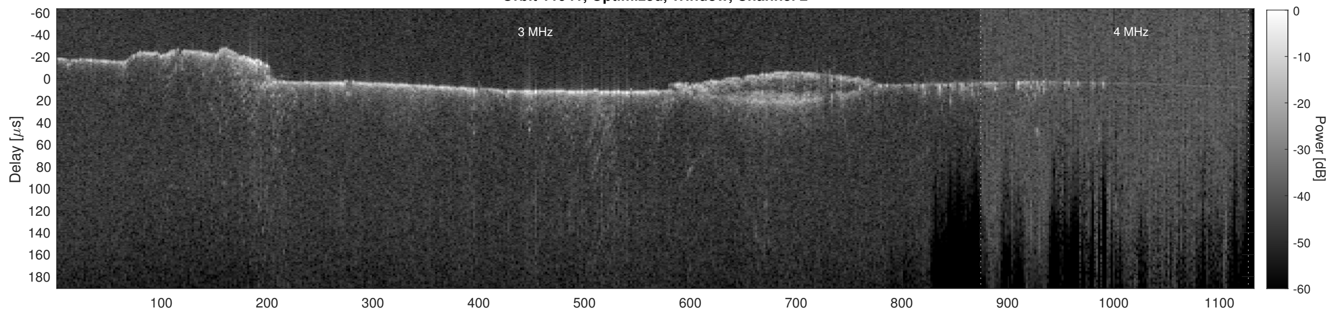
Orbit 11941, Cluttergram
