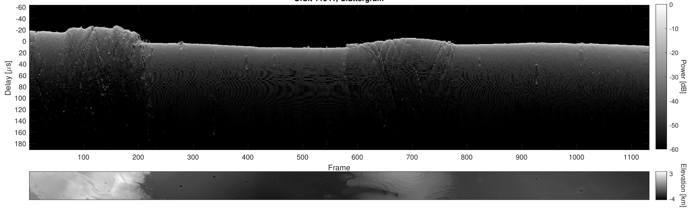
Orbit 11941, Cluttergram
