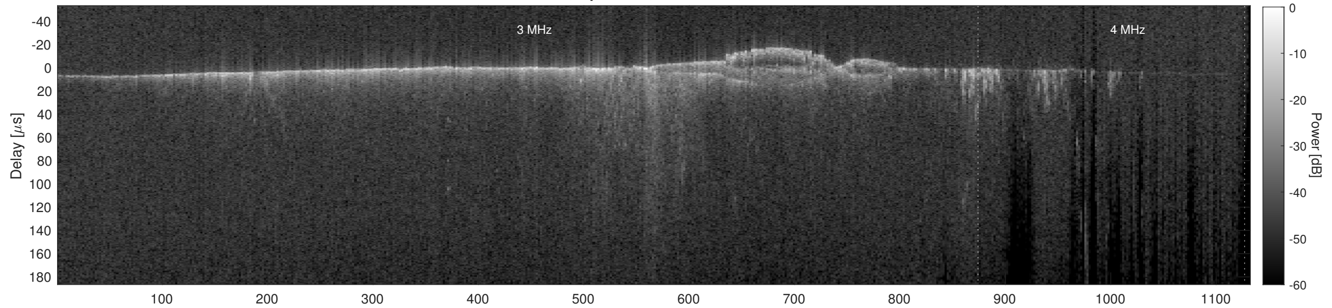
Orbit 11942, Cluttergram
