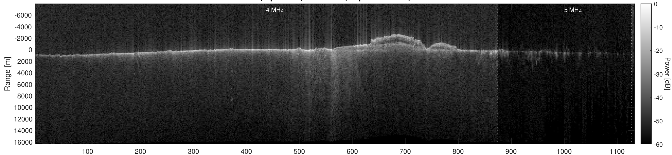
Orbit 11942, Optimized, No Window, Depth-Corrected, Channel 2
