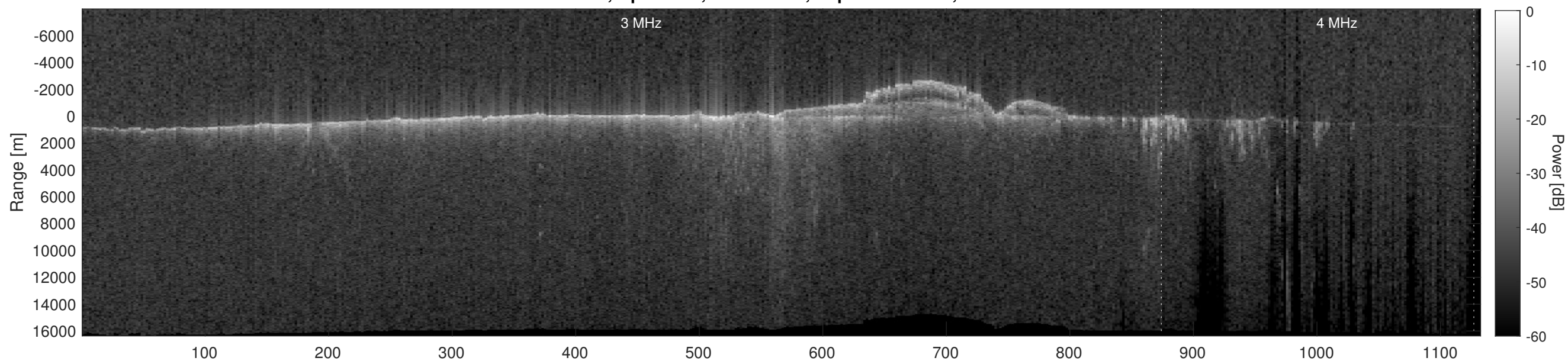
Orbit 11942, Depth-Corrected Cluttergram
