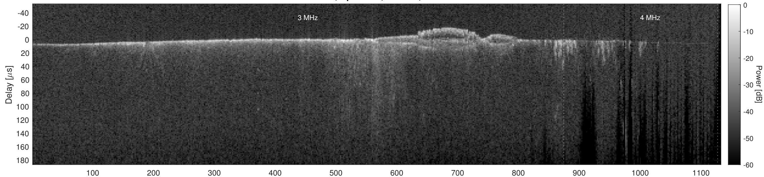
Orbit 11942, Cluttergram
