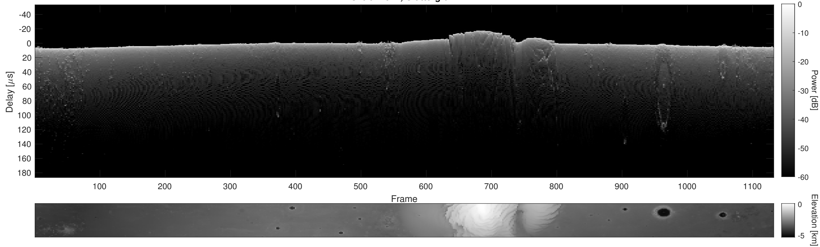
Orbit 11942, Cluttergram
