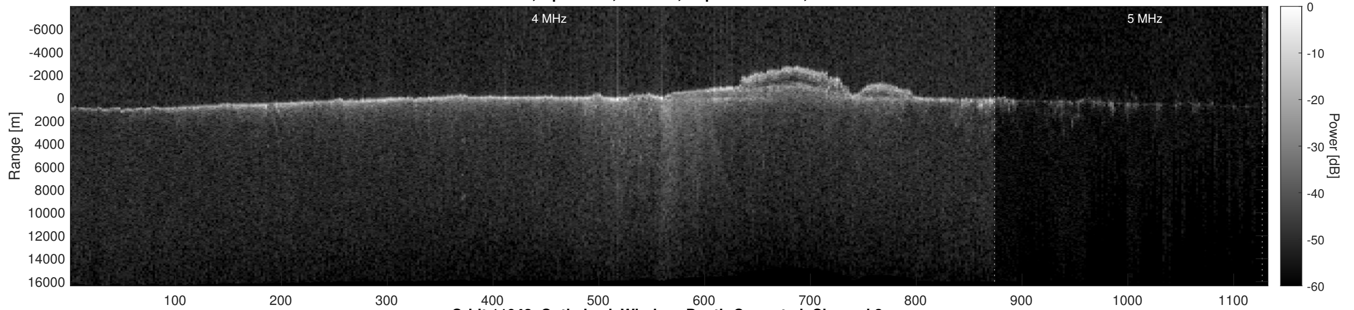
Orbit 11942, Optimized, Window, Depth-Corrected, Channel 2
