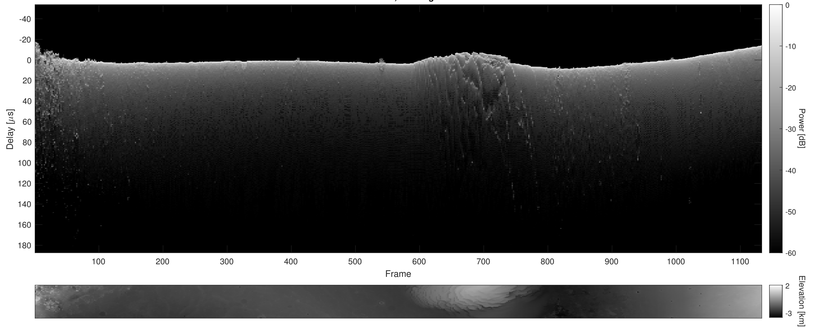
Orbit 11943, Cluttergram
