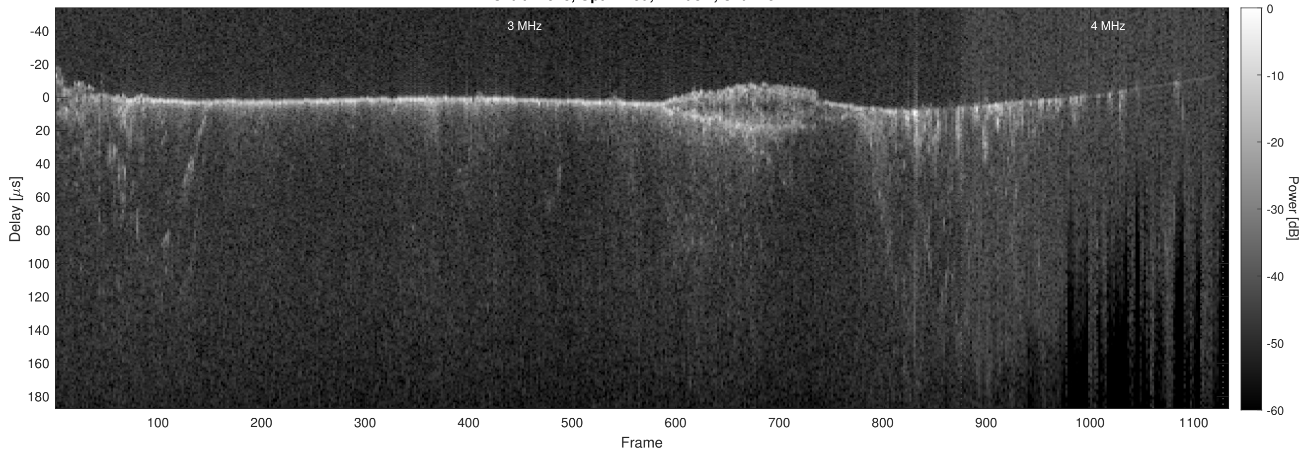
Orbit 11943, Optimized, Window, Channel 2
