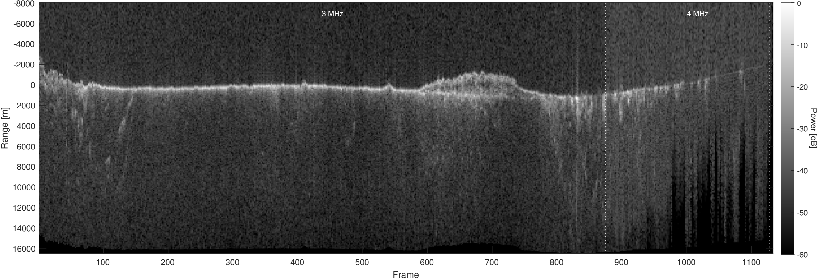
Orbit 11943, Optimized, Window, Depth-Corrected, Channel 2
