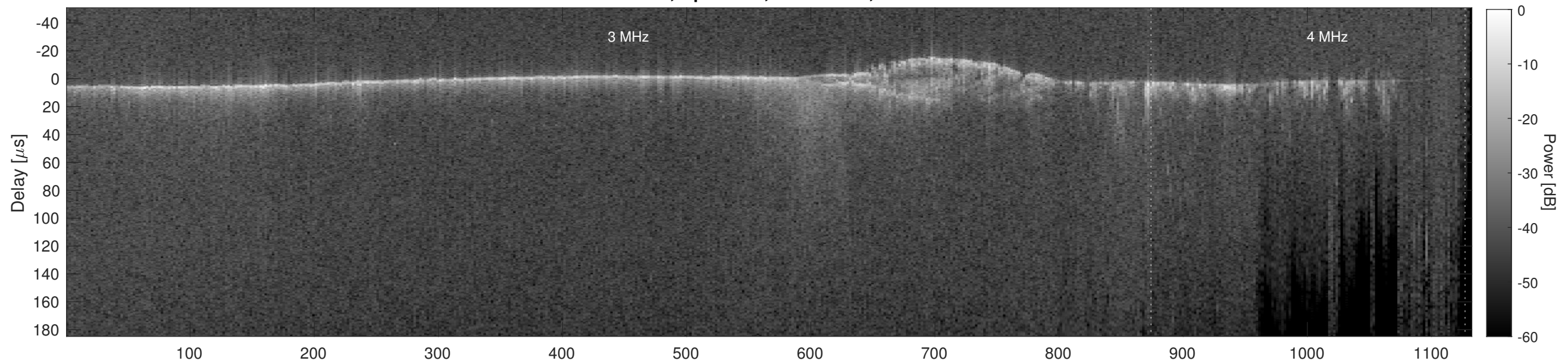
Orbit 11946, Cluttergram
