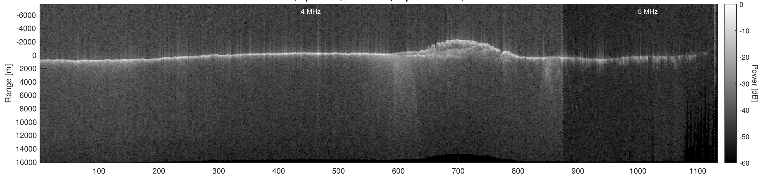
Orbit 11946, Optimized, No Window, Depth-Corrected, Channel 2
