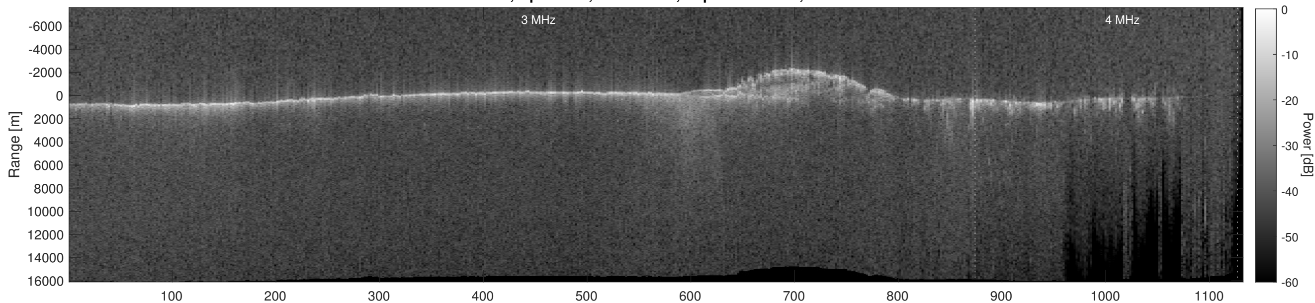
Orbit 11946, Depth-Corrected Cluttergram
