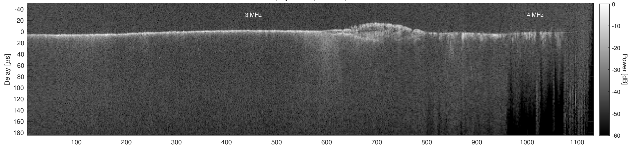
Orbit 11946, Cluttergram
