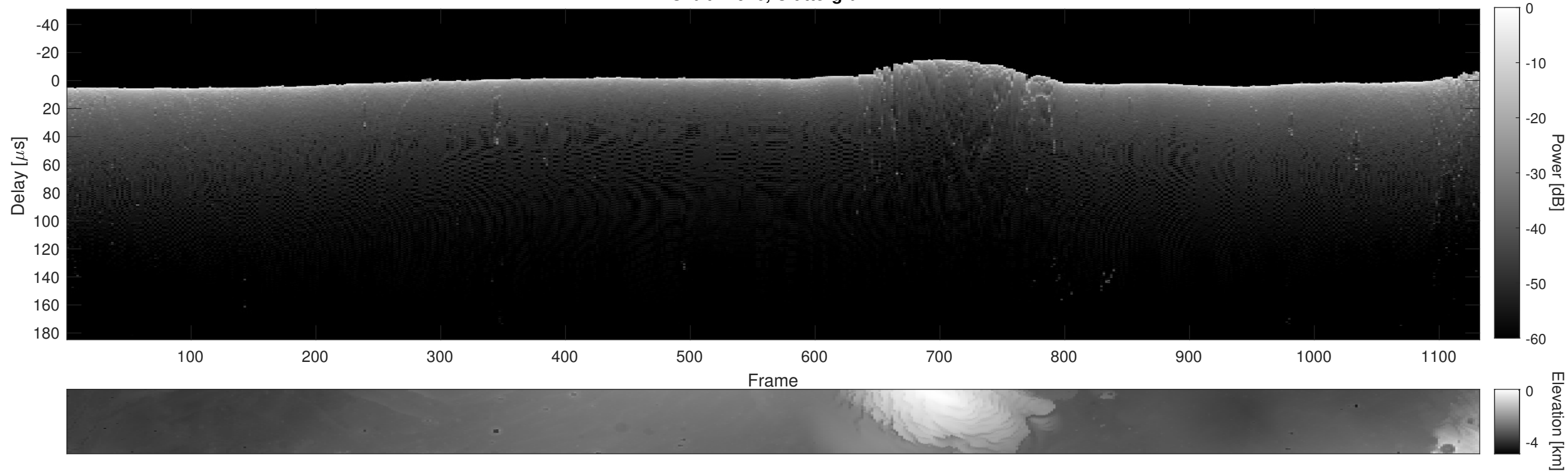
Orbit 11946, Cluttergram
