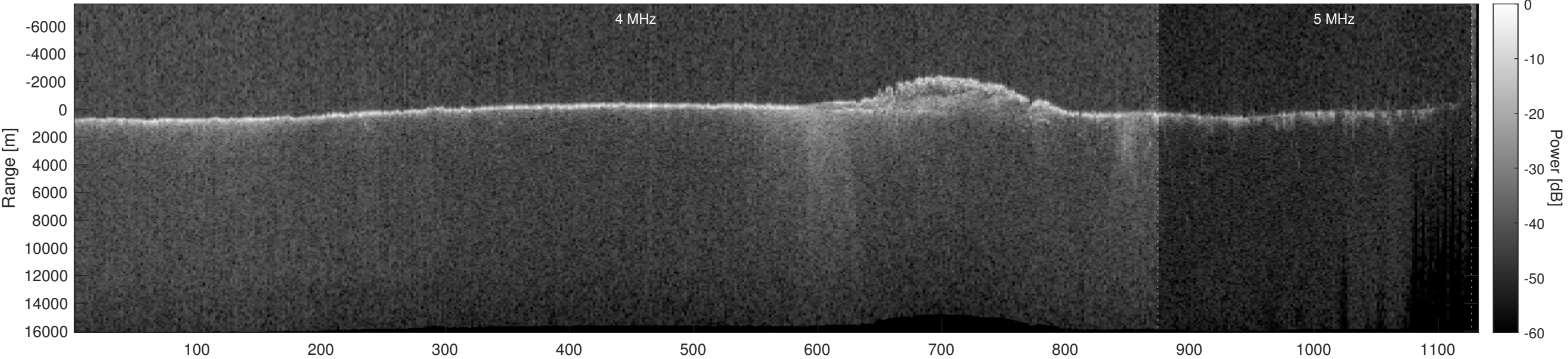
Orbit 11946, Optimized, Window, Depth-Corrected, Channel 2
