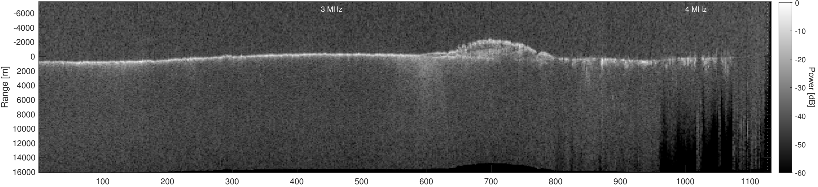
Orbit 11946, Depth-Corrected Cluttergram
