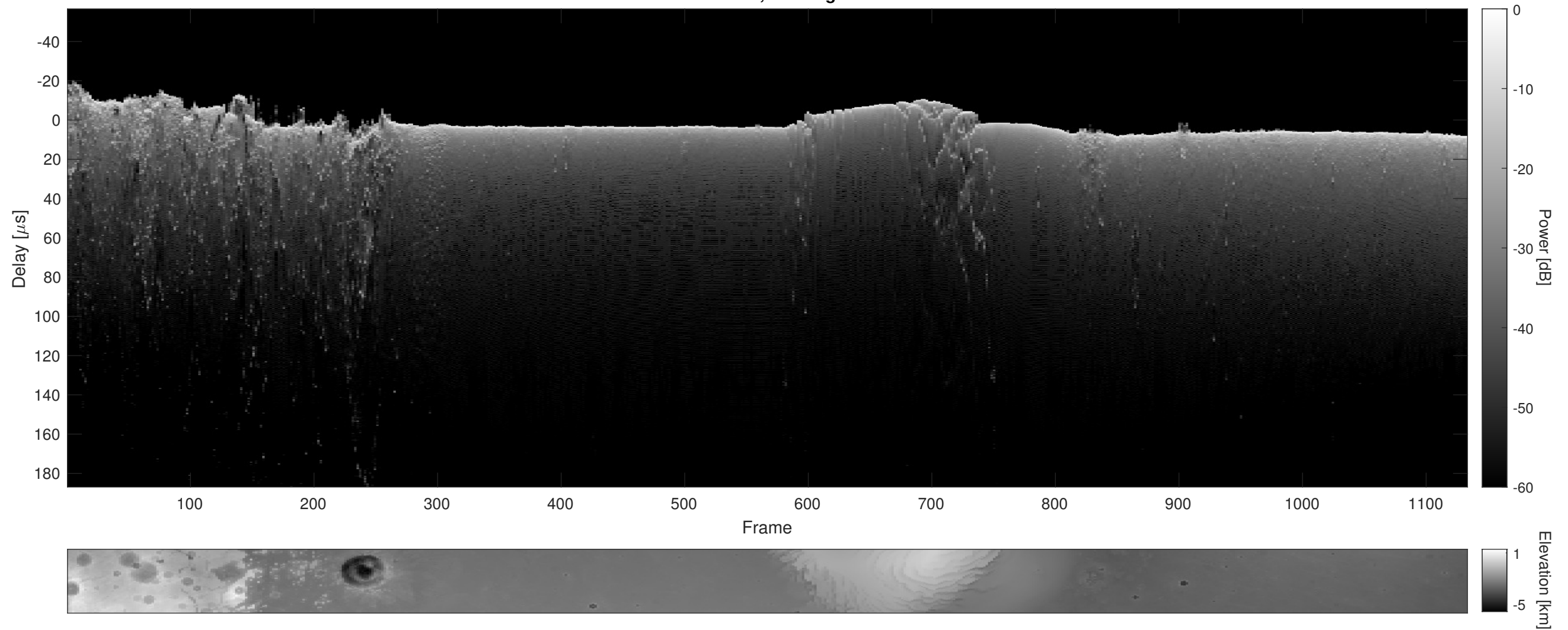
Orbit 11947, Cluttergram
