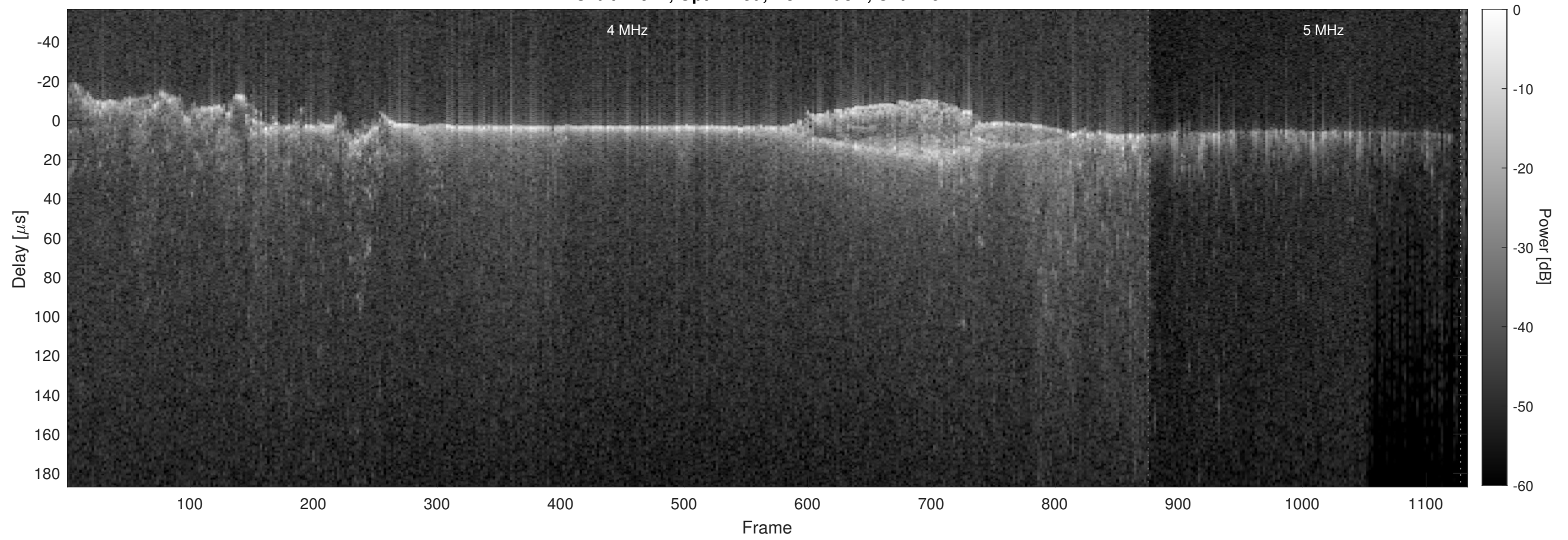
Orbit 11947, Optimized, No Window, Channel 2
