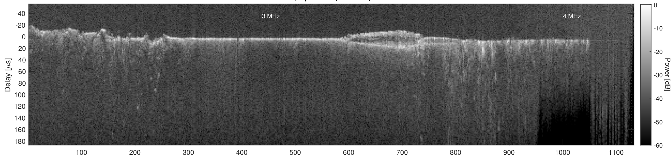
Orbit 11947, Cluttergram
