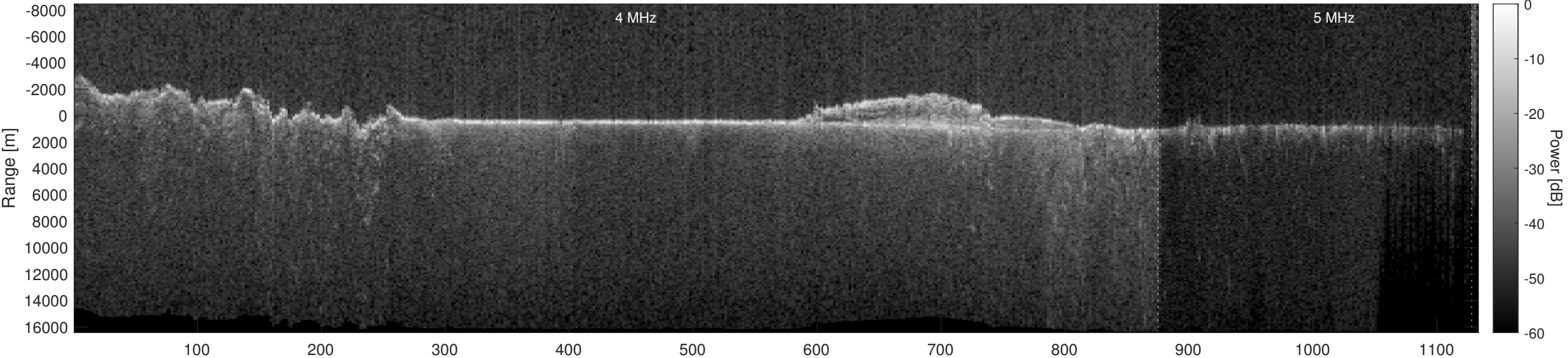
Orbit 11947, Optimized, Window, Depth-Corrected, Channel 2
