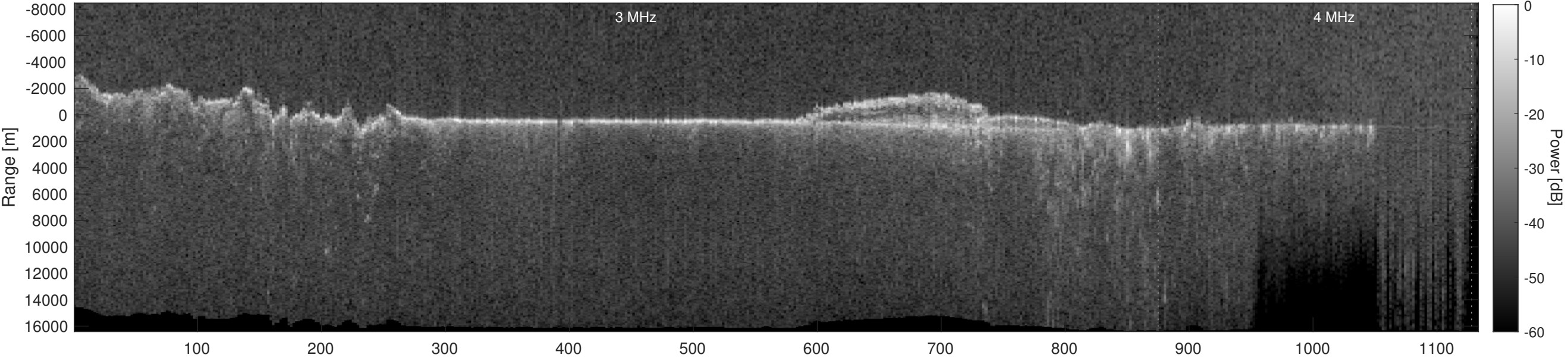
Orbit 11947, Depth-Corrected Cluttergram
