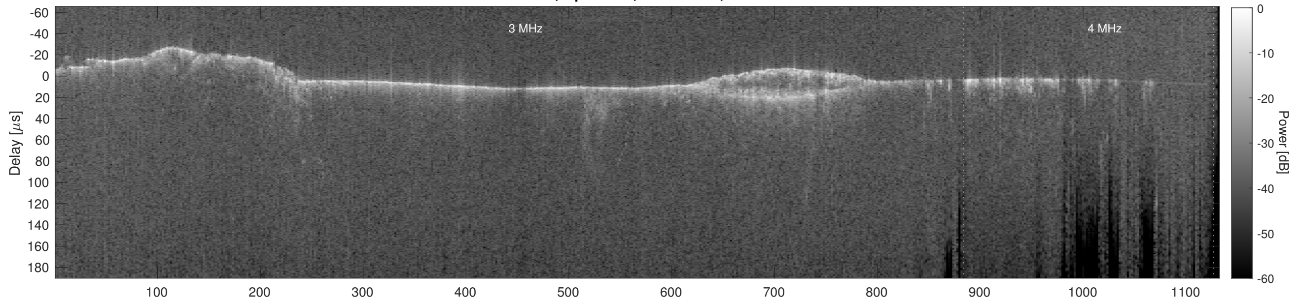
Orbit 11948, Cluttergram
