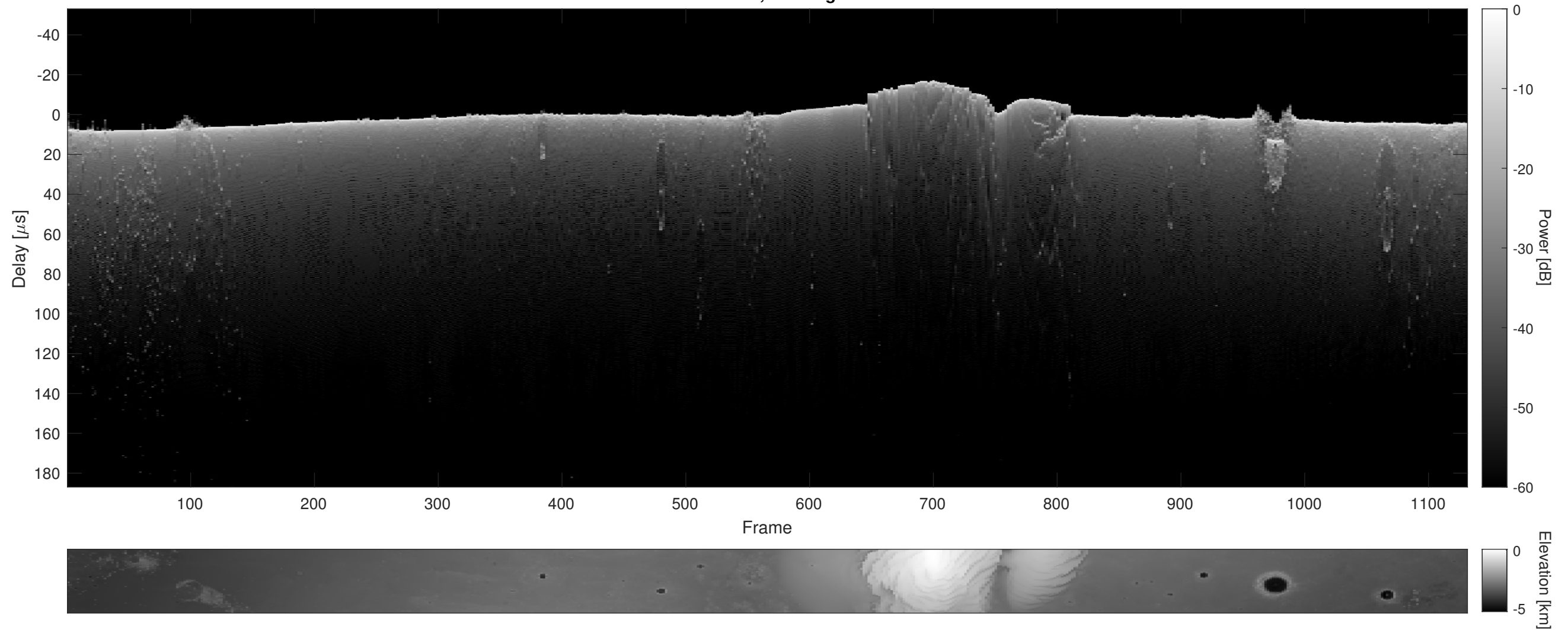
Orbit 11949, Cluttergram
