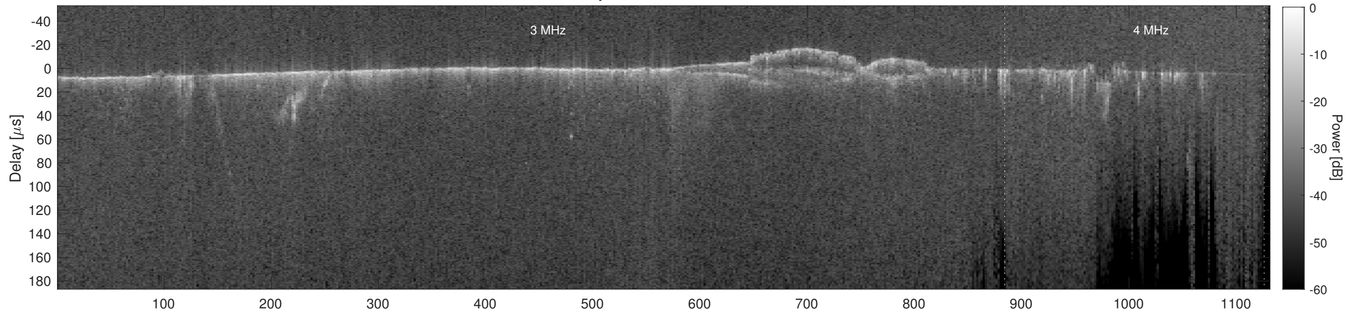
Orbit 11949, Cluttergram
