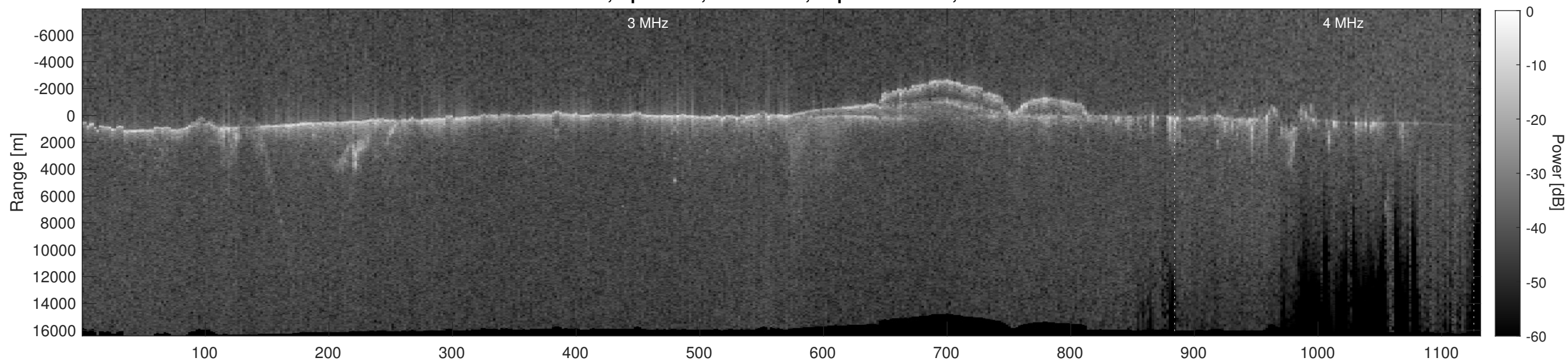
Orbit 11949, Depth-Corrected Cluttergram
