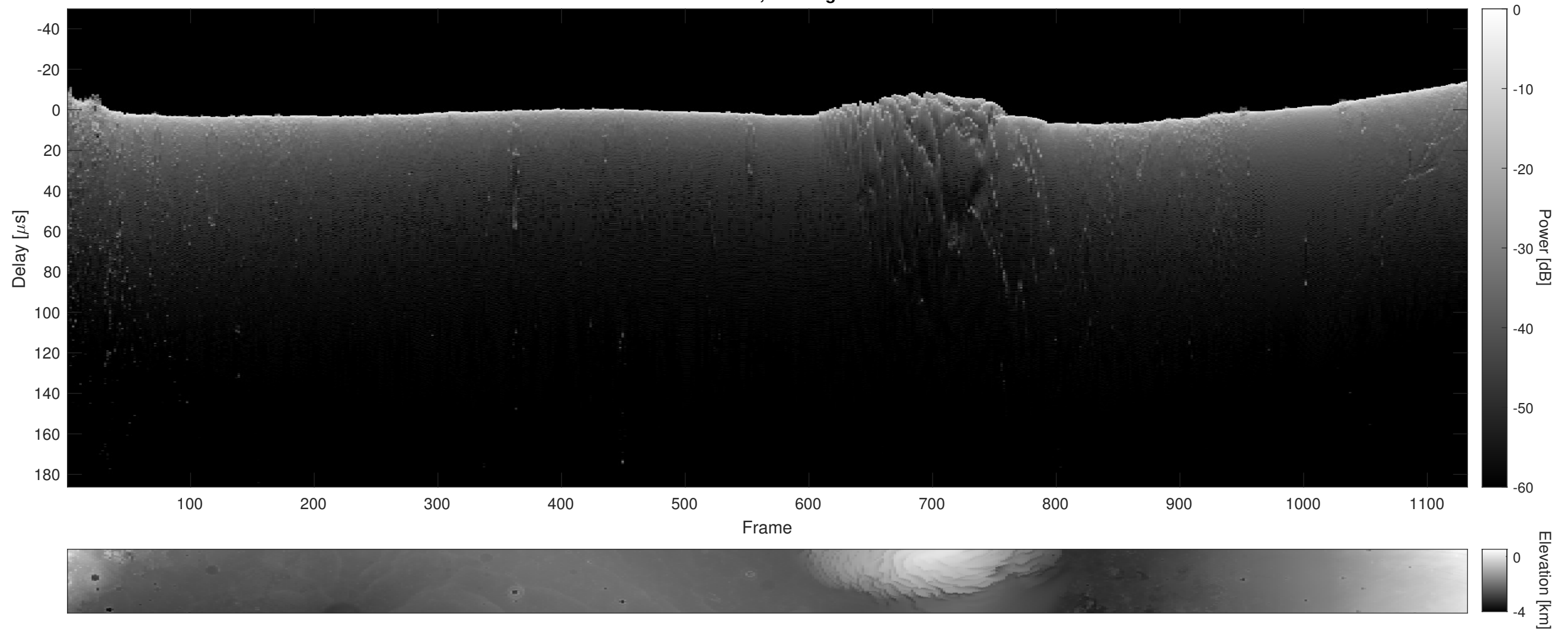
Orbit 11950, Cluttergram
