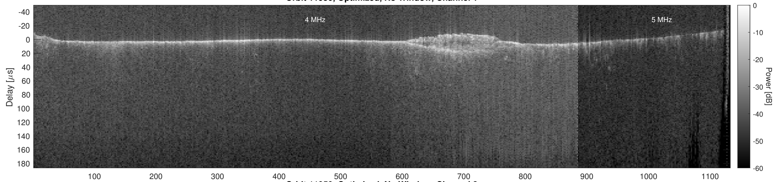
Orbit 11950, Optimized, No Window, Channel 2
