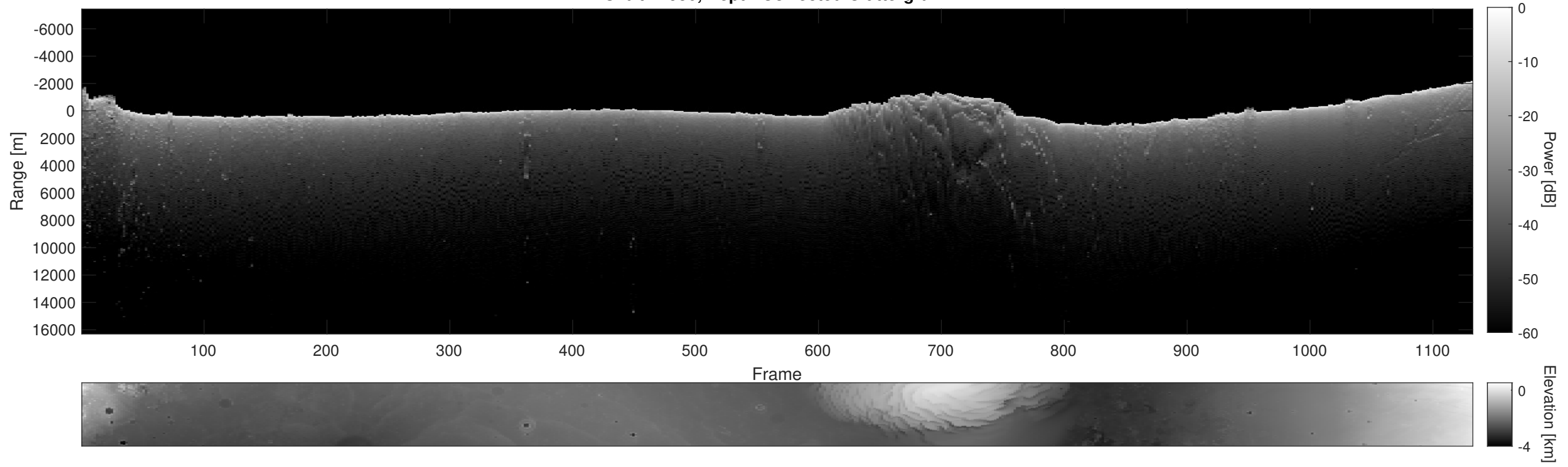
Orbit 11950, Depth-Corrected Cluttergram
