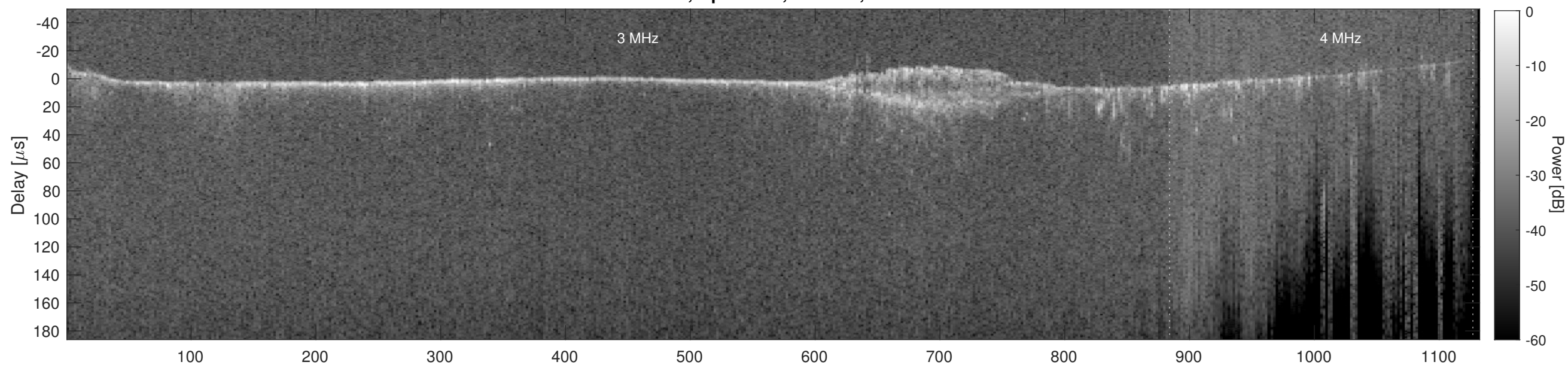
Orbit 11950, Cluttergram
