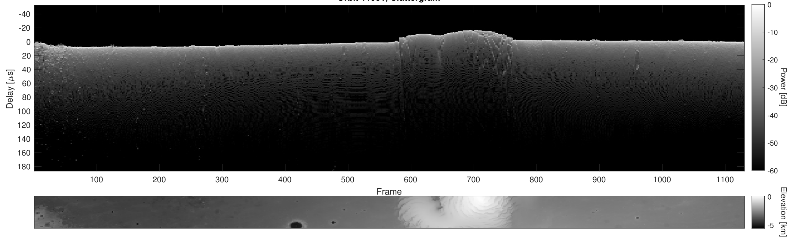
Orbit 11951, Cluttergram
