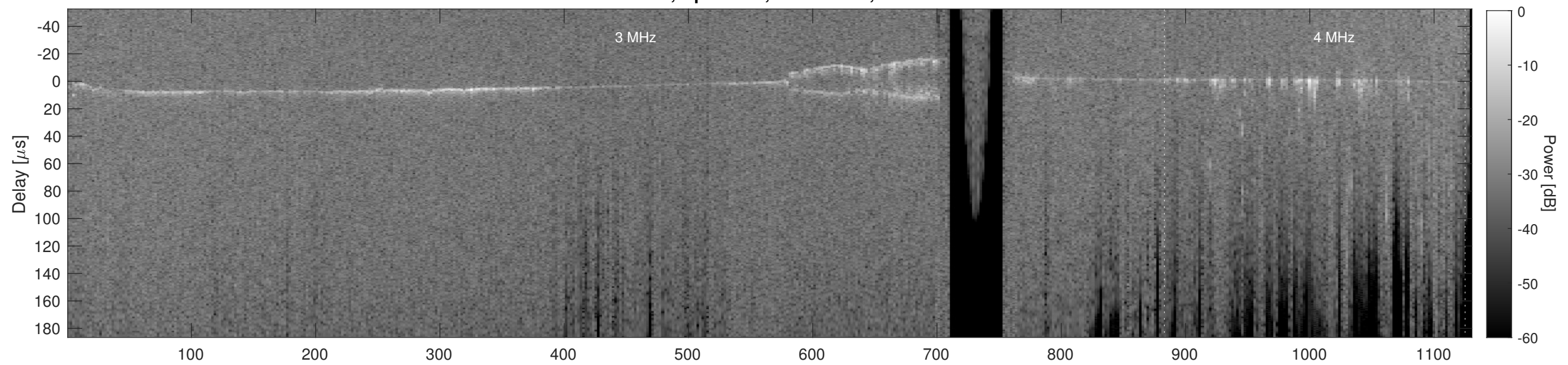
Orbit 11951, Cluttergram
