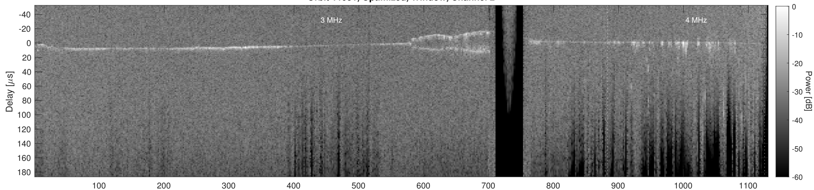
Orbit 11951, Cluttergram
