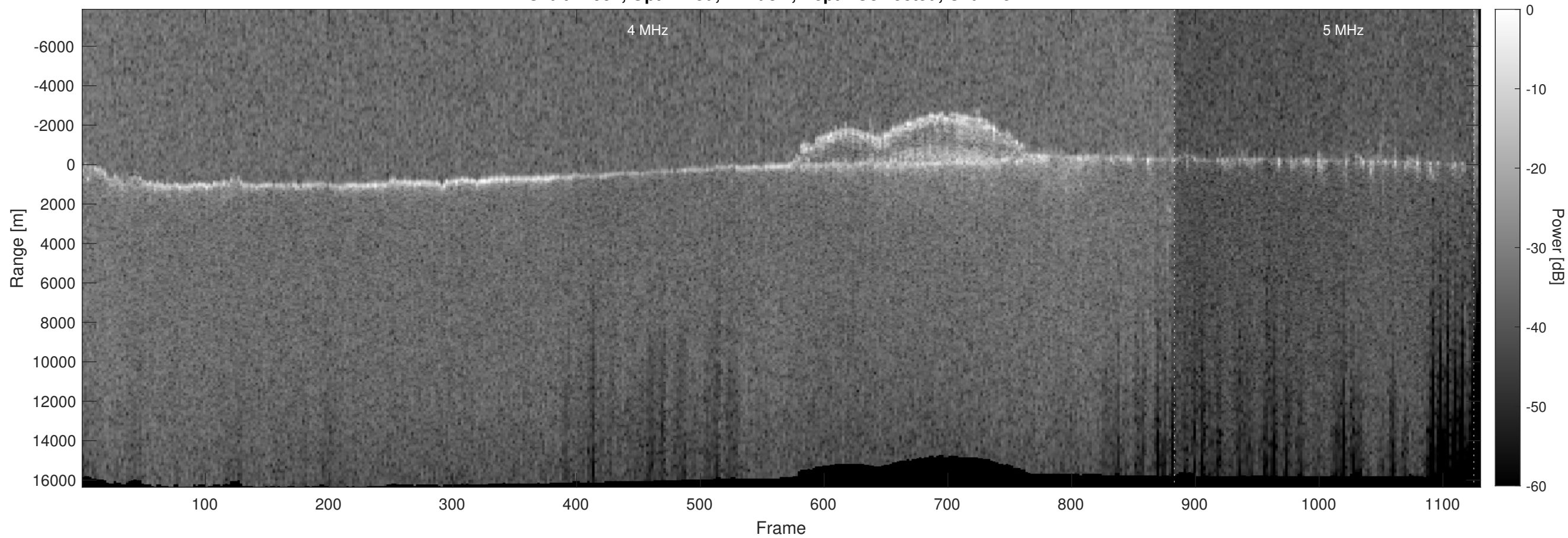
Orbit 11951, Optimized, Window, Depth-Corrected, Channel 2
