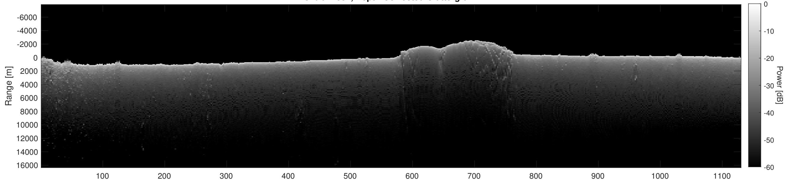
Orbit 11951, Depth-Corrected Cluttergram
