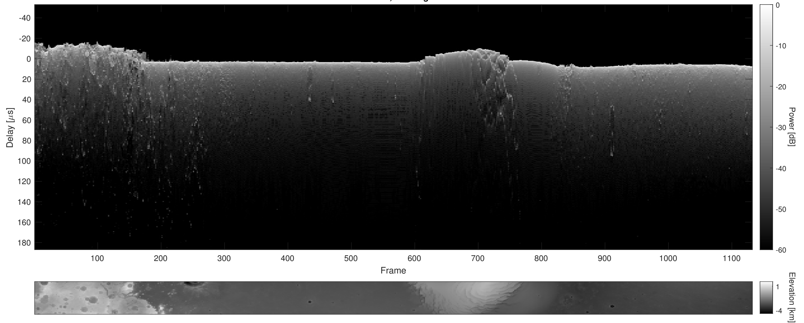
Orbit 11954, Cluttergram
