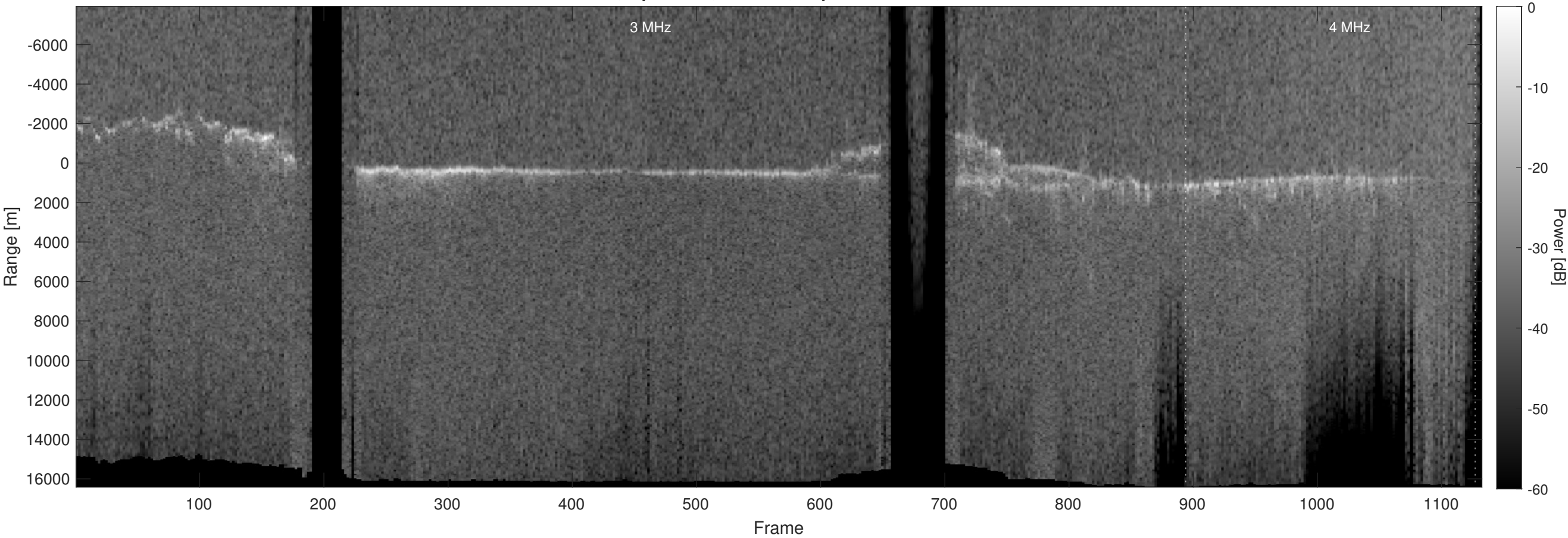
Orbit 11954, Optimized, Window, Depth-Corrected, Channel 2
