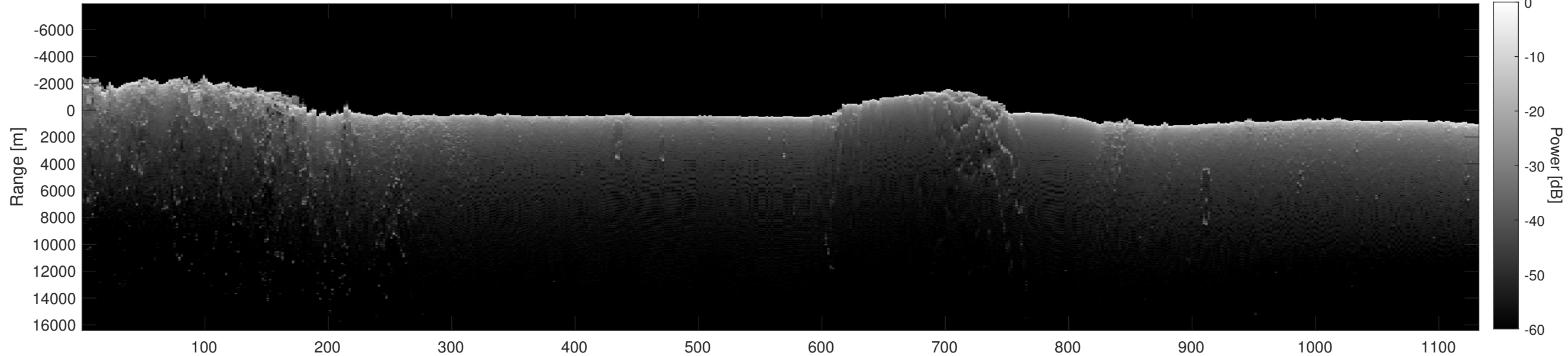
Orbit 11954, Depth-Corrected Cluttergram
