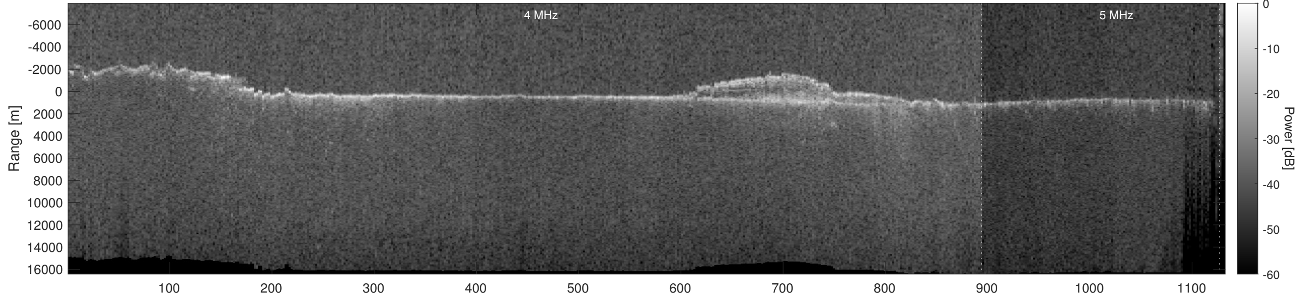
Orbit 11954, Optimized, Window, Depth-Corrected, Channel 2
