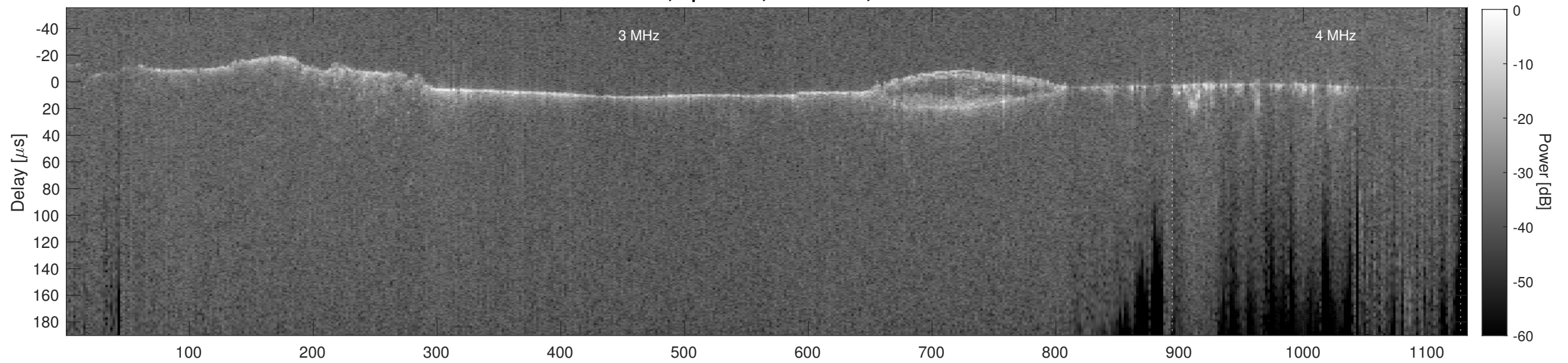
Orbit 11955, Cluttergram
