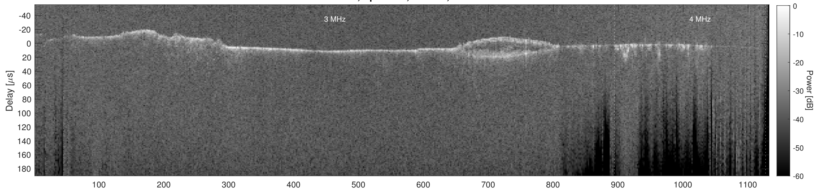
Orbit 11955, Cluttergram
