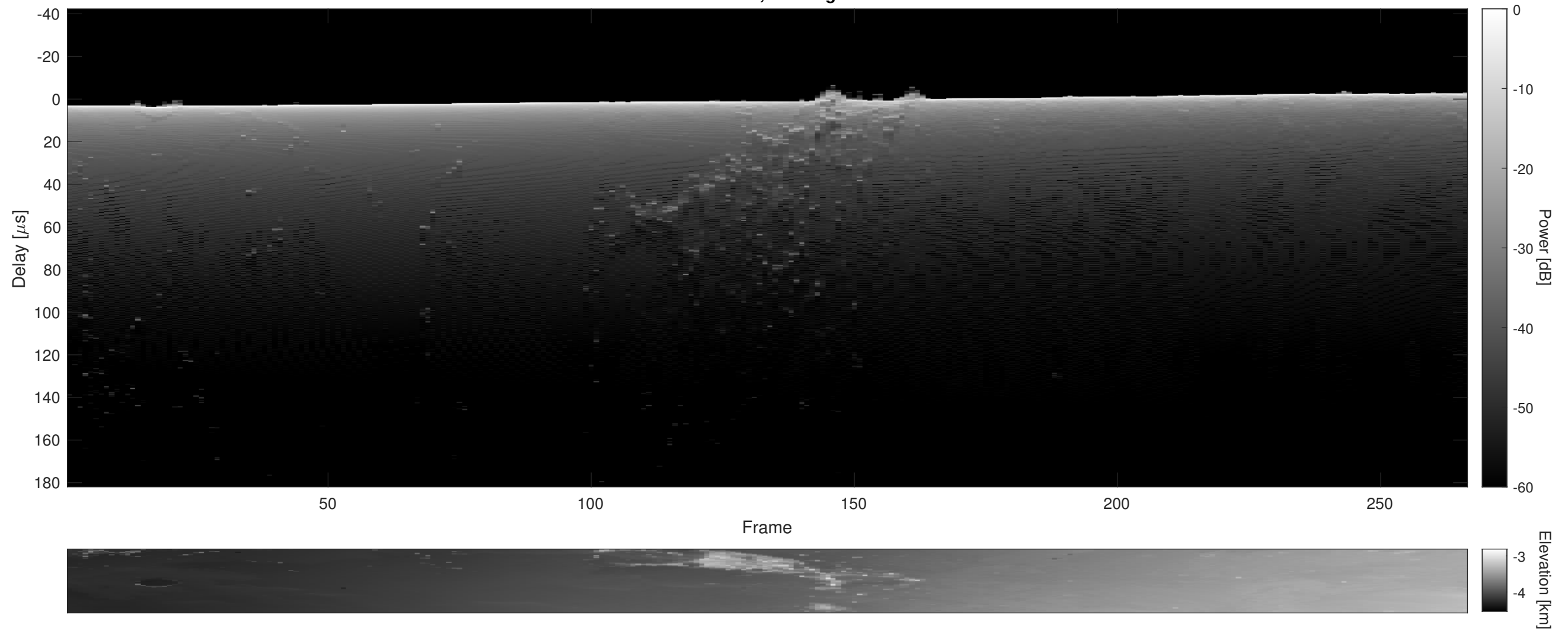
Orbit 11956, Cluttergram
