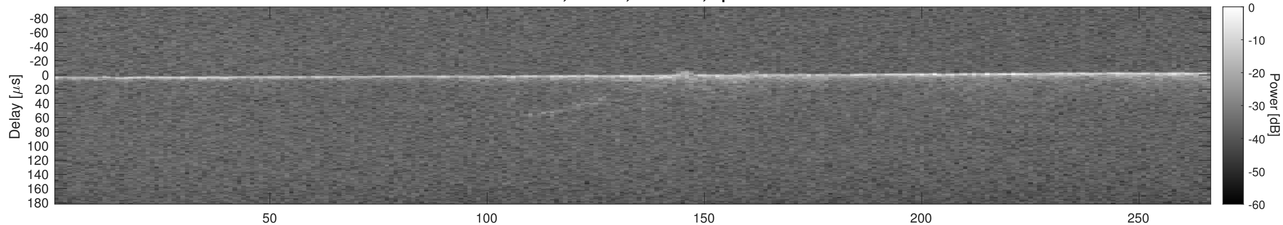
Orbit 11956, Cluttergram
