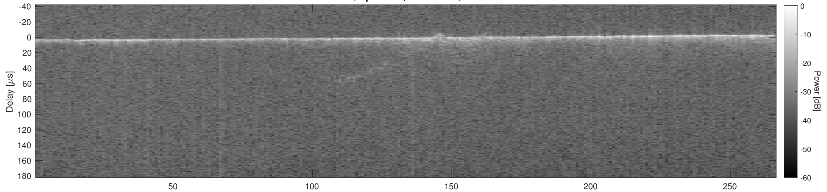
Orbit 11956, Cluttergram
