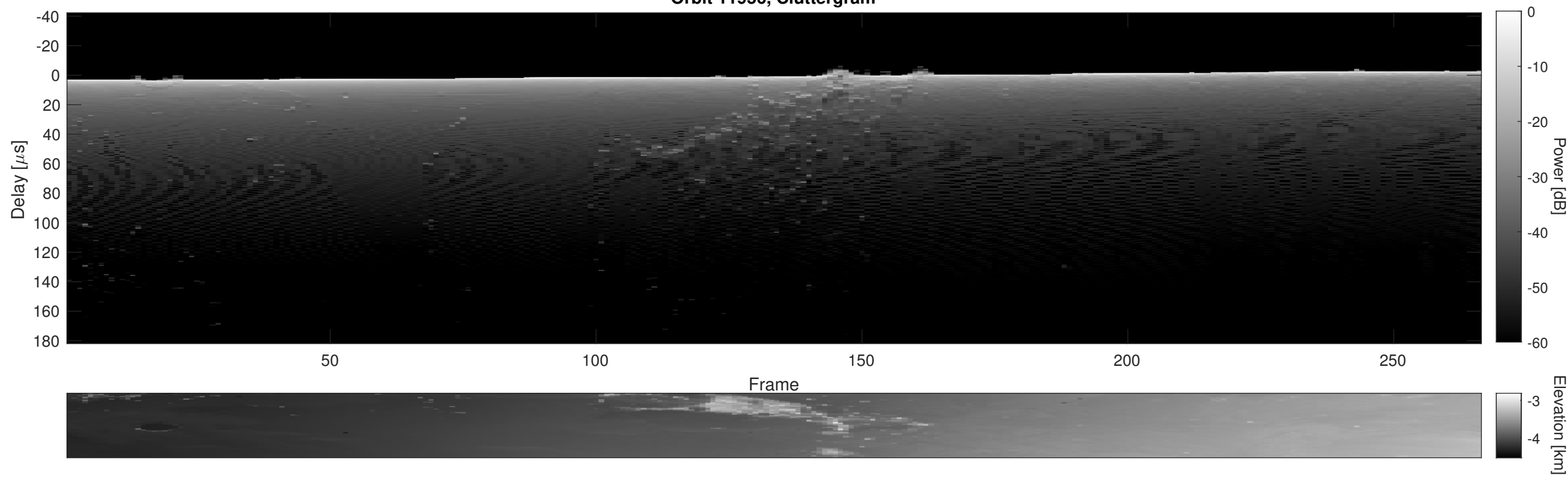
Orbit 11956, Cluttergram
