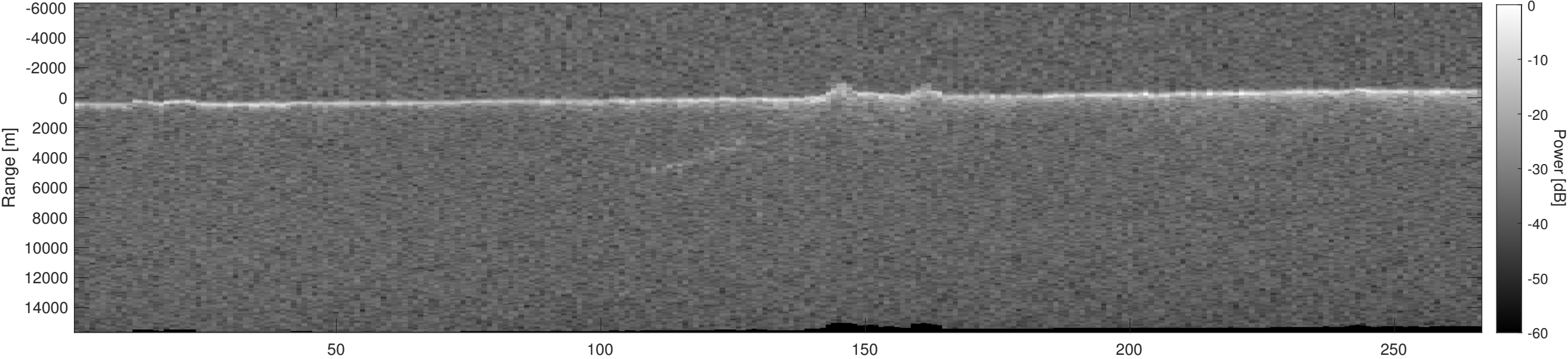
Orbit 11956, Depth-Corrected Cluttergram
