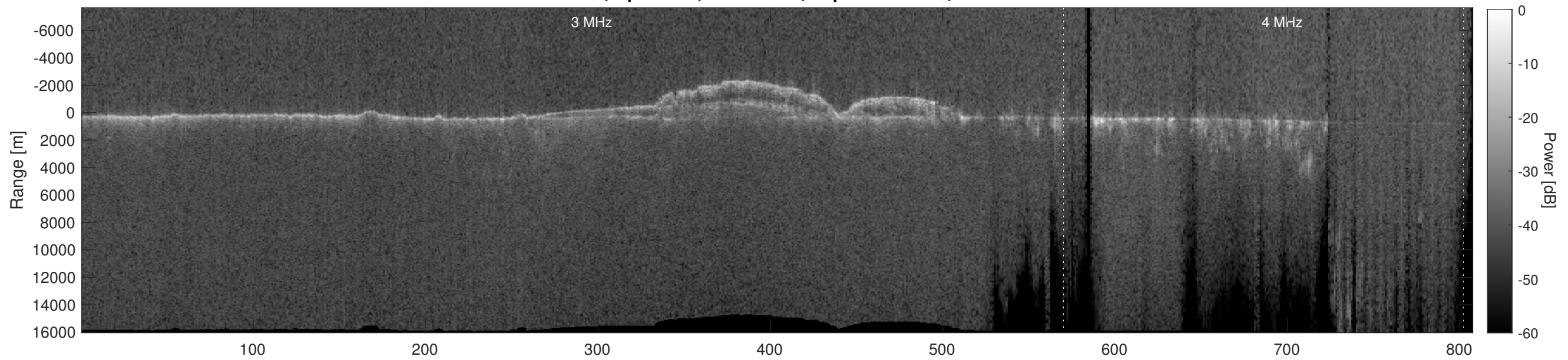
Orbit 11958, Depth-Corrected Cluttergram
