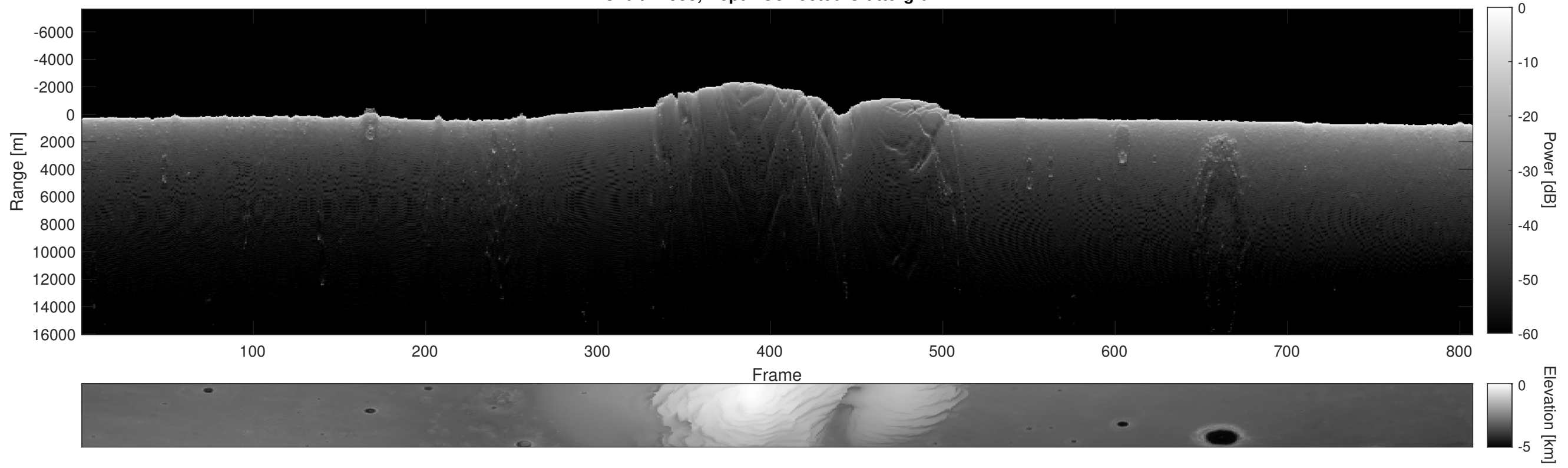
Orbit 11958, Depth-Corrected Cluttergram
