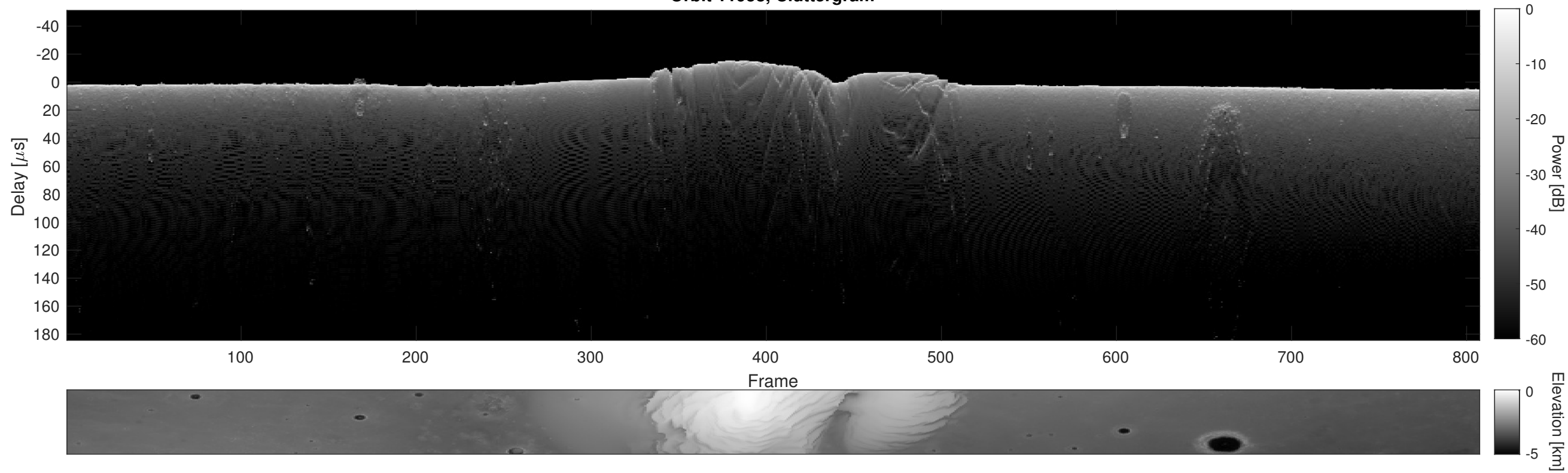
Orbit 11958, Cluttergram
