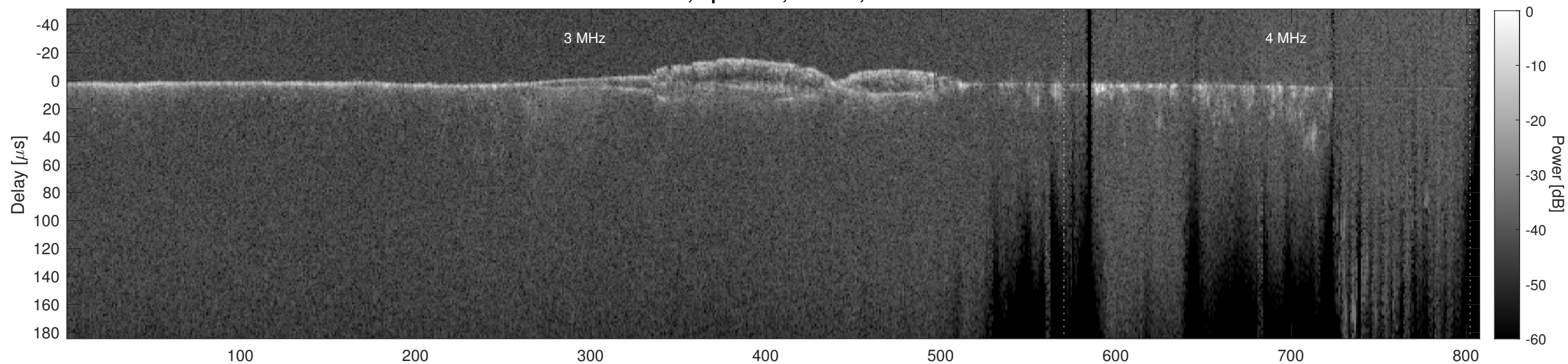
Orbit 11958, Cluttergram
