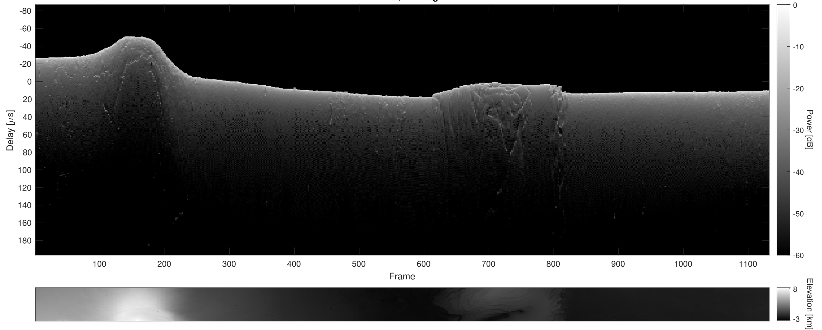
Orbit 11959, Cluttergram
